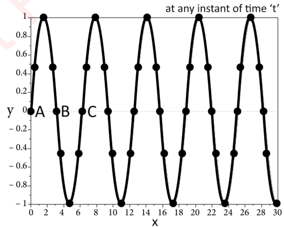
Fig. 1.8 Particles in same and different phases
