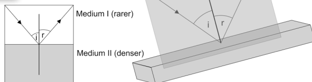
Fig. 2.1 Phenomenon of reflection
