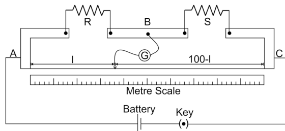
Fig 4.13 Meter bridge
