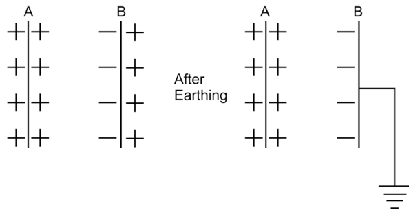
Fig 3.14 Capacitor
