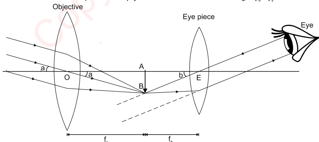
Fig. 2.12 Astronomical telescope
