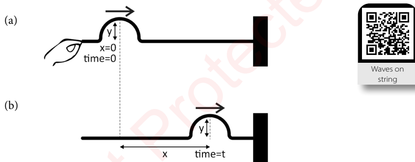
Fig. 1.7 Propagation of disturbance
