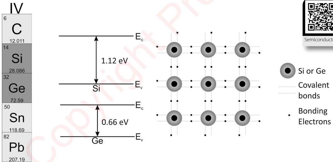
Fig 6.4 Covalent bond in Si and Ge
