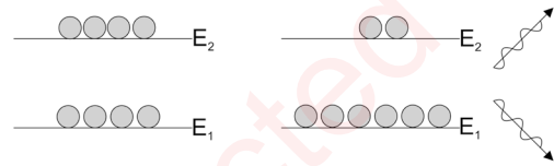
Fig 7.3 Spontaneous Emission
