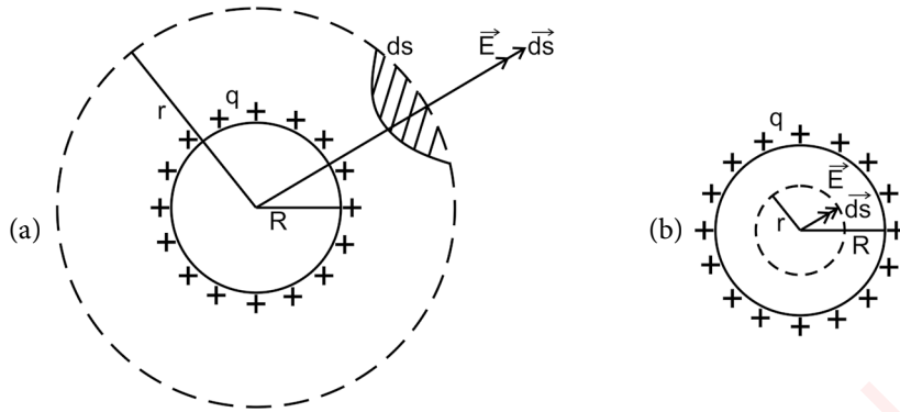
Fig 3.13 Electric field due to uniformly charged sphere
