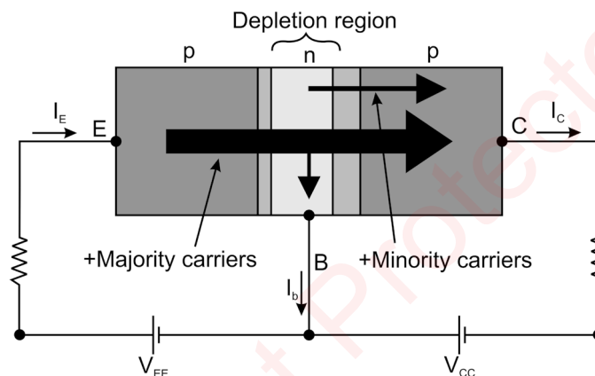
Fig 6.13 Operation of transistor
