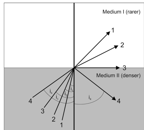
Fig. 2.8 Total internal reflection
