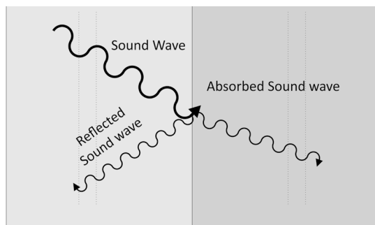
Fig. 1.13 Absorption of sound wave
