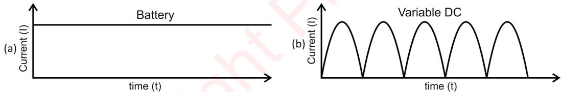
Fig. 4.5 Direct current
