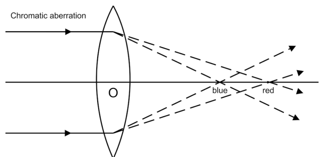
Fig. 2.4 Chromatic aberration
