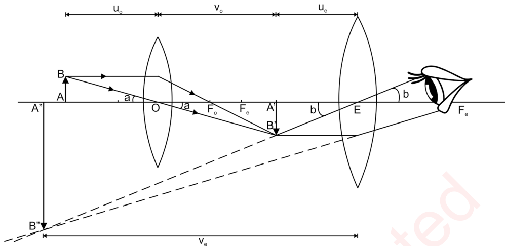
Fig. 2.11 Compound microscope
