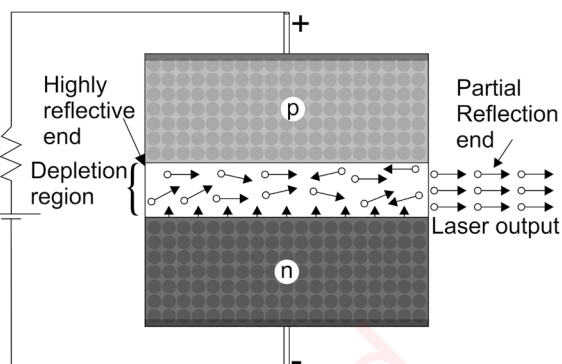
Fig 7.11 Diode laser
