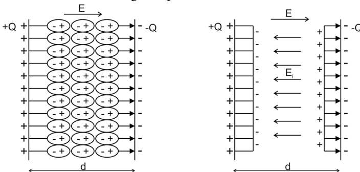
Fig 3.20 Dielectrics in capacitor
