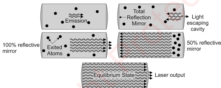
Fig 7.8 Optical resonator
