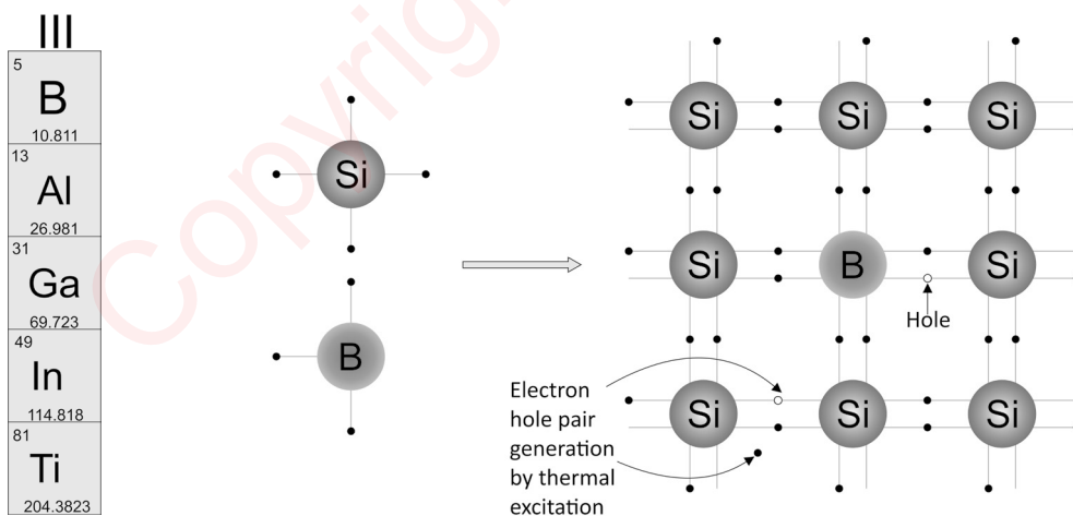
Fig 6.5 p type semiconductor
