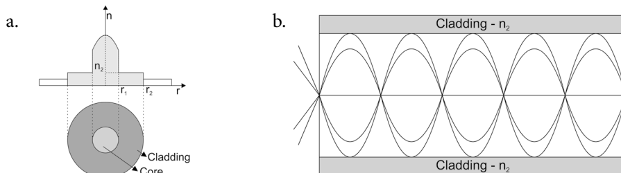
Fig 7.17 Refractive index profile and light propagation Graded index fiber
