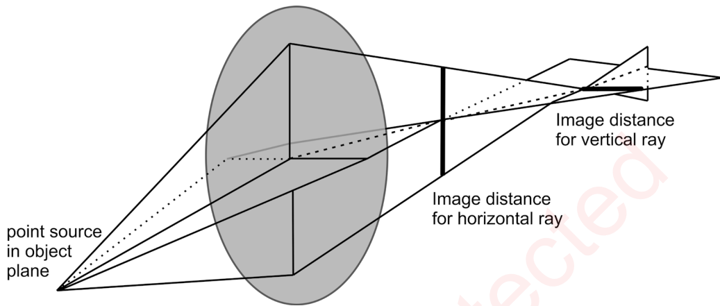
Fig. 2.7 Astigmatism
